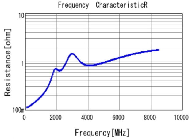
■ GRM1552C1H101JA01 R DCOV, 20degC
