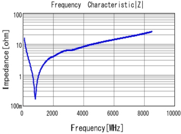
■ GRM1552C1H101JA01 |Z| DCOV, 20degC
