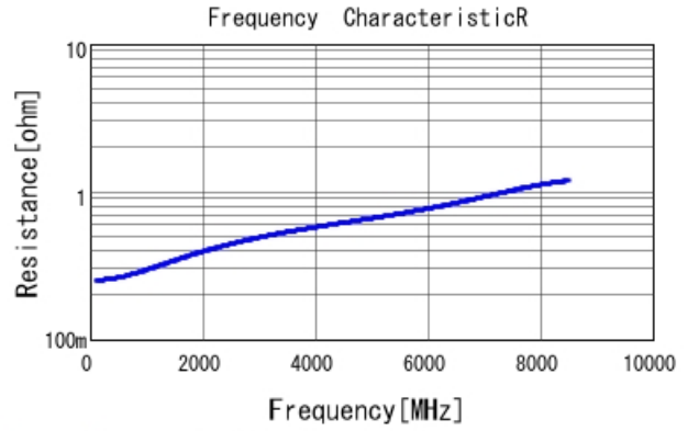
GRM0335C1H3R0BA01 R DCOV, 25degC
