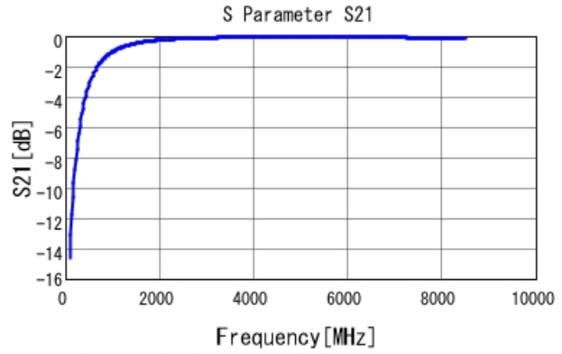
GRM0335C1H3R0BA01 S21 DCOV, 25degC
