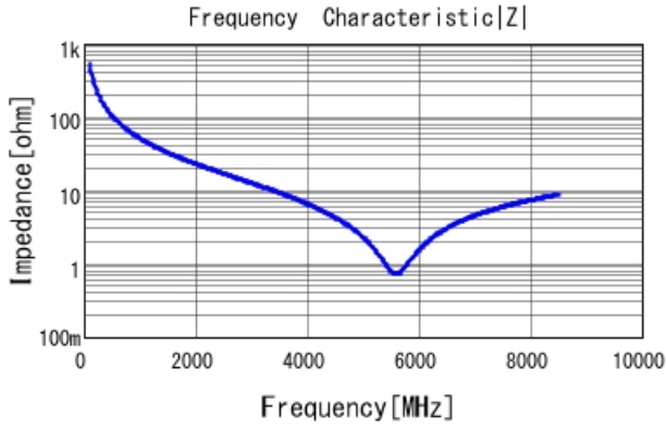
GRM0335C1H3R0BA01 |Z| DCOV, 25degC
