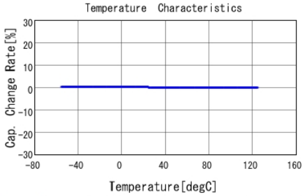
GRM0335C1H3R0BA01 C-Temp. capchange, DCOV, AC1Vrms
