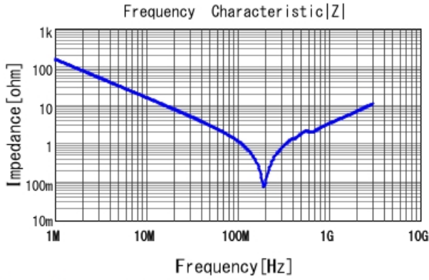
GRM21A7U2E102JW31 |Z| DCOV, 25degC
