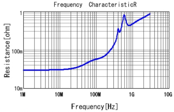
GRM21A7U2E102JW31 R DCOV, 25degC
