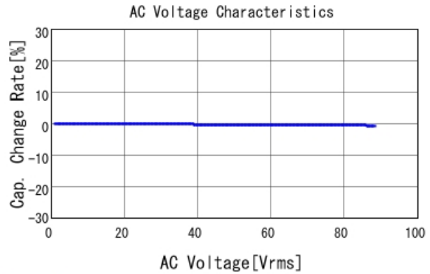
GRM21A7U2E102JW31 C-AC Voltage capchange, DCOV, 25
