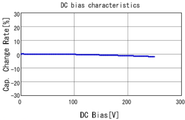
GRM21A7U2E102JW31 C-DC bias capchange, 25.0degC, A
