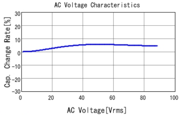
GRM21A7U2E121JW31 C-AC Voltage capchange, DCOV, 25
