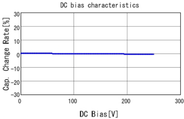
GRM21A7U2E121JW31 C-DC bias capchange, 25.0degC, A
