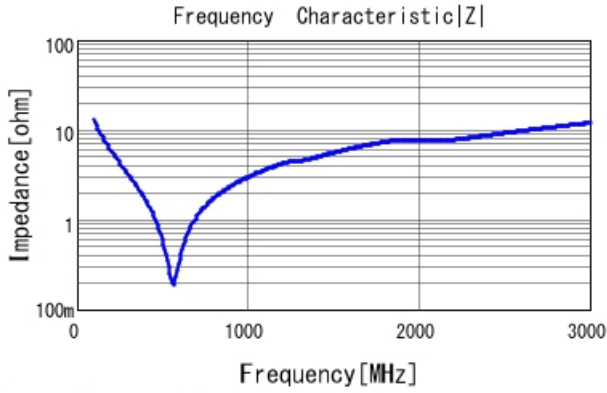
GRM21A7U2E121JW31 |Z| DCOV, 25degC
