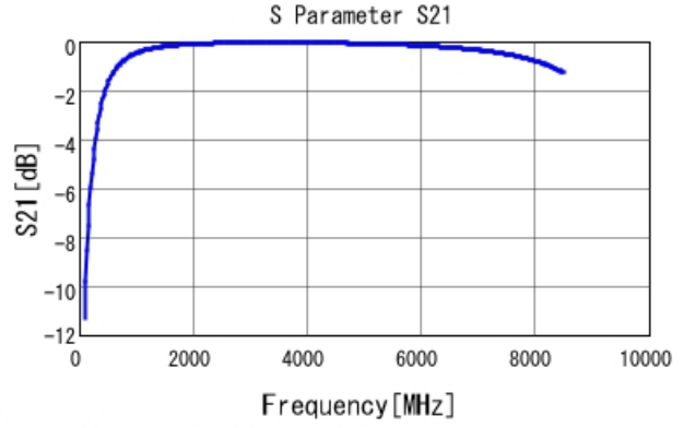
GRM1555C1H4R5BA01 S21 DC0V, 25degC
