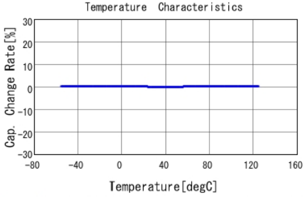
GRM1555C1H4R5BA01 C-Temp. capchange, DC0V, AC1Vrms
