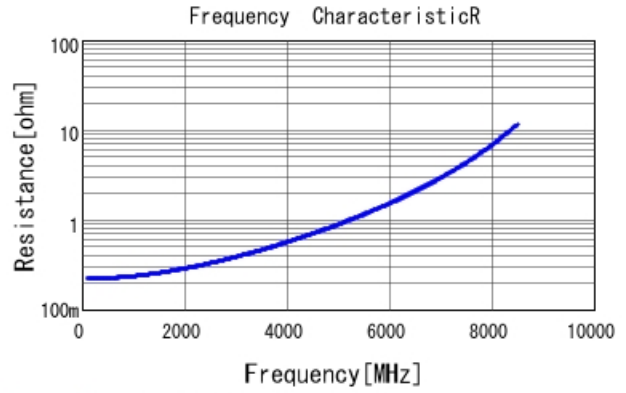
GRM1555C1H4R5BA01 R DCOV, 25degC
