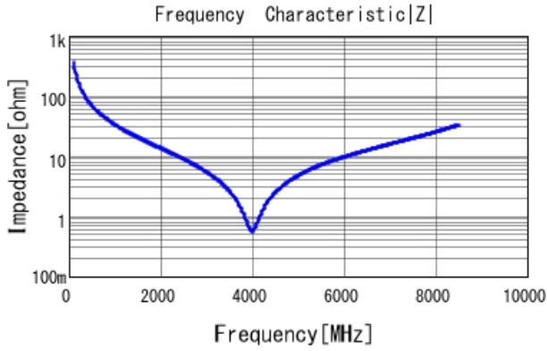
GRM1555C1H4R5BA01 |Z| DCOV, 25degC
