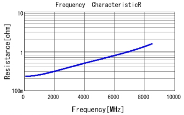
■ GRM0335C2A4R2BA01 R DCOV, 25degC
