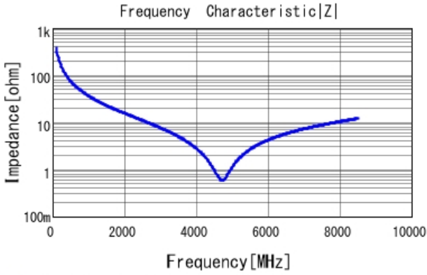
■ GRM0335C2A4R2BA01 |Z| DCOV, 25degC
