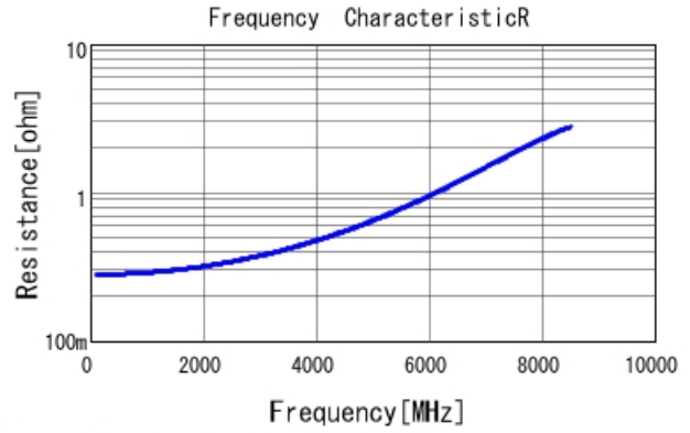
GRM1555C2A3R0CA01 R DCOV, 25degC
