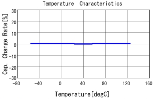
GRM1555C2A3R0CA01 C-Temp. capchange, DCOV, AC1Vrms
