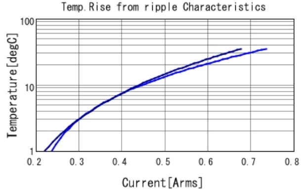
GRM1555C2A3R0CA01 Temp. rise — 2GHz — 3GHz
