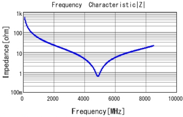
GRM1555C2A3R0CA01 |Z| DCOV, 25degC
