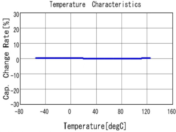
■ GRM1882C1H562JA01 C-Temp. capchange, DCOV, AC1Vrms
