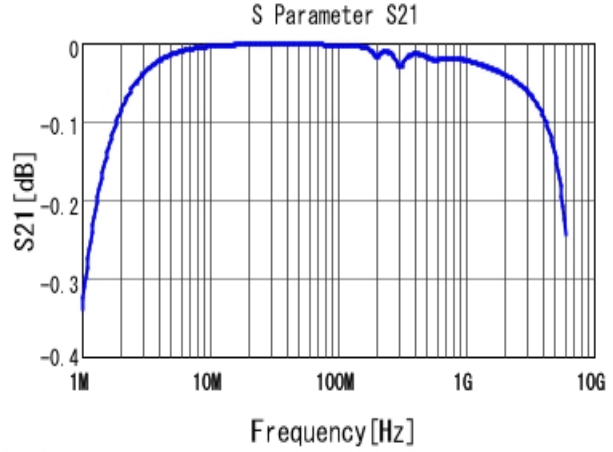
■ GRM1882C1H562JA01 S21 DCOV, 20degC
