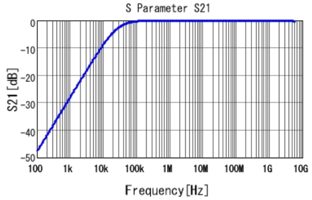
■ GCJ188R92A683KA01 S21 DCOV, 25degC
