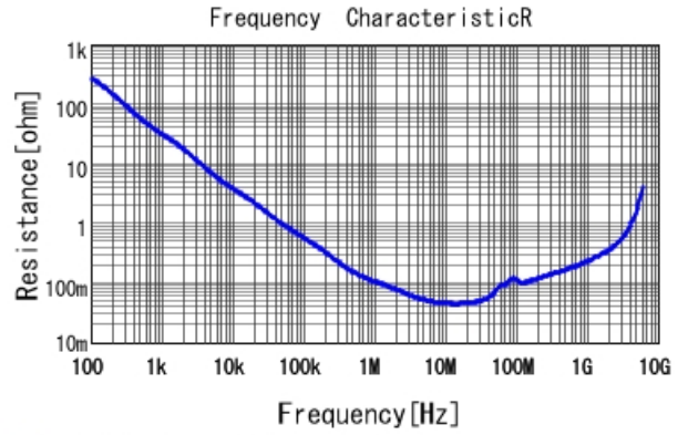
■ GCJ188R92A683KA01 R DCOV, 25degC
