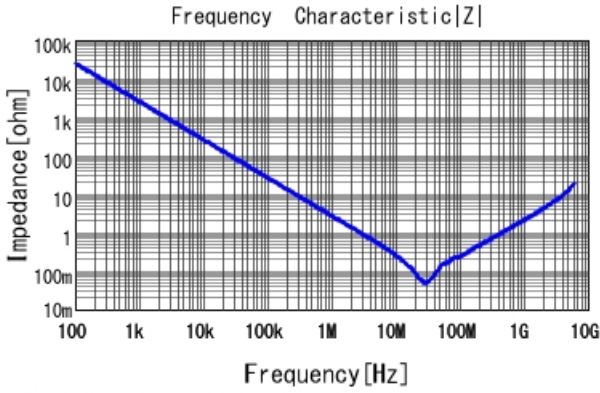
■ GCJ188R92A683KA01 |Z| DCOV, 25degC
