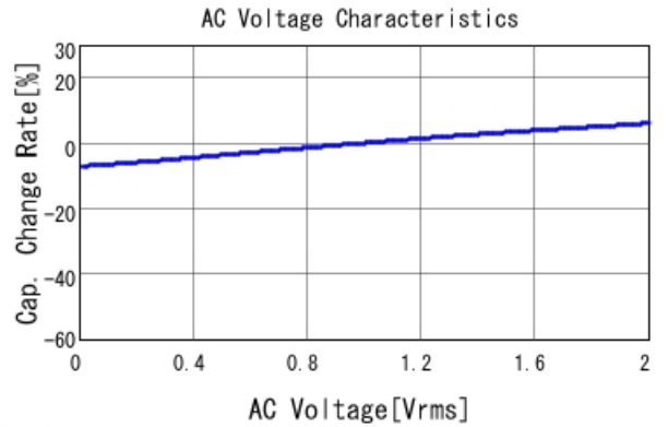
■ GCJ188R92A683KA01 C-AC Voltage capchange, DCOV, 25.0d
