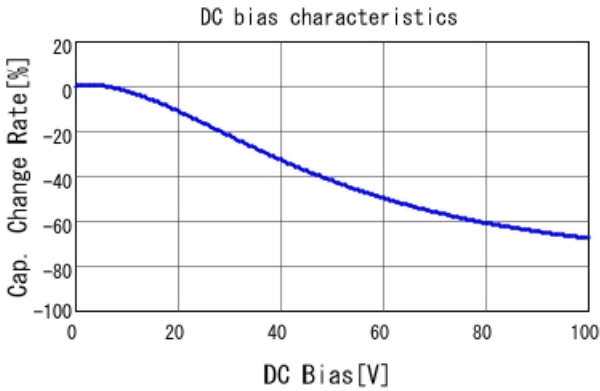
■ GCJ188R92A683KA01 C-DC bias capchange, 25.0degC, AC1.
