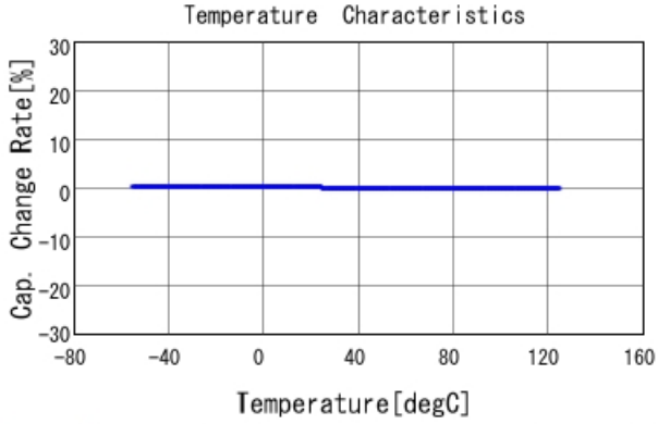
GRM2165C2A271JA01 C-Temp. capchange, DCOV, AC1Vrms
