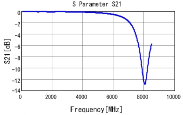
GRM2165C2A271JA01 S21 DCOV, 25degC
