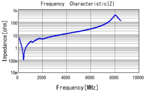
GRM2165C2A271JA01 |Z| DCOV, 25degC
