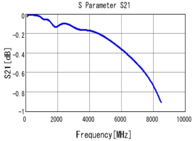
■ GRM1885C1H221JA01 S21 DCOV, 25degC
