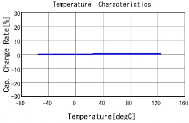
GRM1885C2AR50BA01 C-Temp. capchange, DCOV, AC1Vrms
