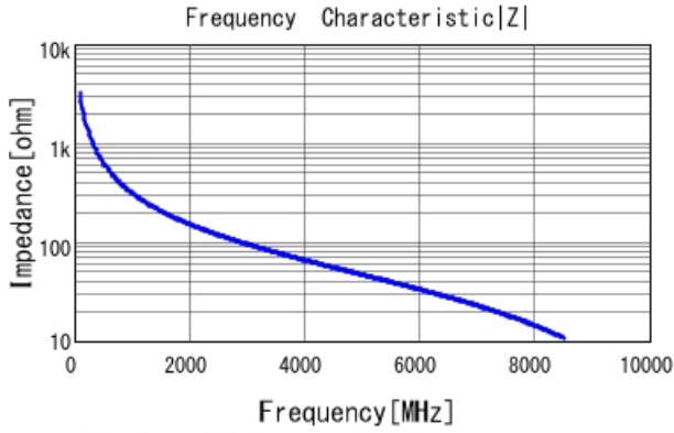
GRM1885C2AR50BA01 |Z| DCOV, 25degC
