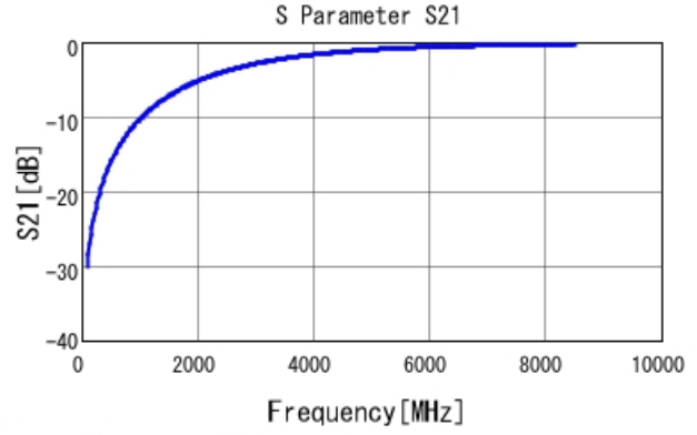
GRM1885C2AR50BA01 S21 DCOV, 25degC
