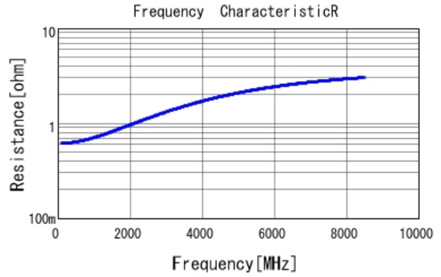
GRM1885C2AR50BA01 R DCOV, 25degC
