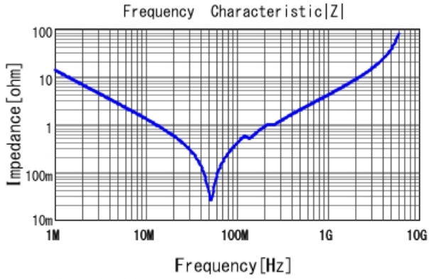
GCM3195C1H123JA16 |Z| DCOV, 25degC
