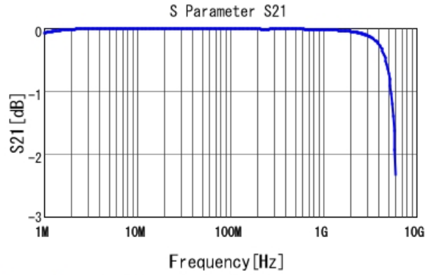
GCM3195C1H123JA16 S21 DCOV, 25degC
