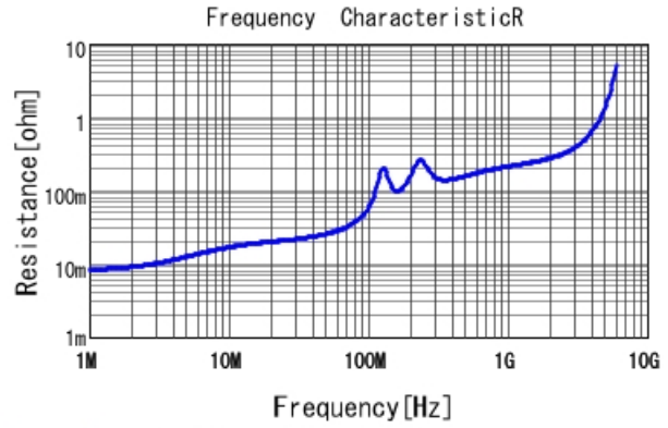
GCM3195C1H123JA16 R DCOV, 25degC
