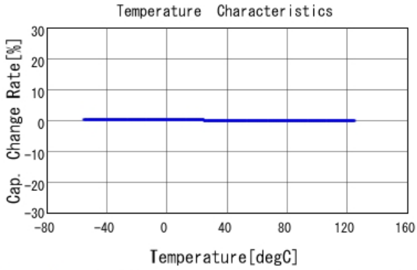
GCM3195C1H123JA16 C-Temp. capchange, DCOV, AC1Vrms
