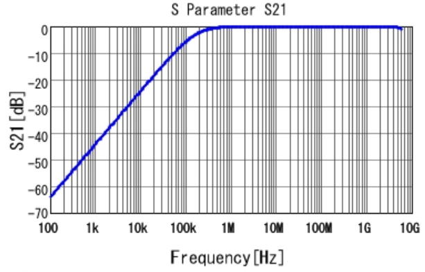
■ GCD188R71H103KA01 S21 DCOV, 25degC
