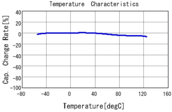
■ GCD188R71H103KA01 C-Temp. capchange, DCO. 0V, AC1. 0Vrm
