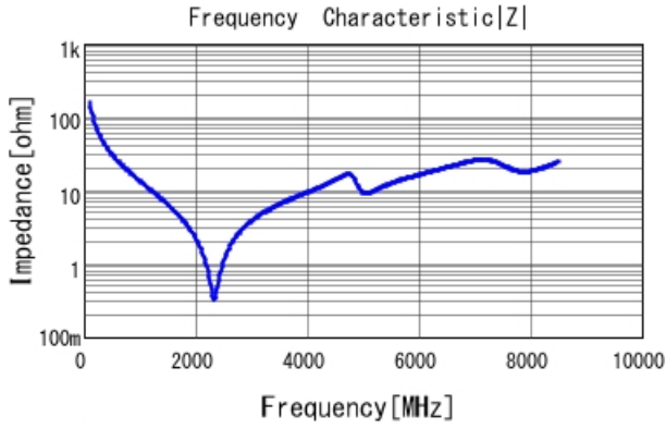
GRM1885C2A9R7BA01 |Z| DCOV, 25degC
