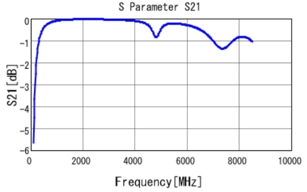
GRM1885C2A9R7BA01 S21 DCOV, 25degC
