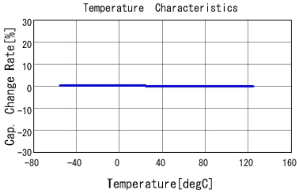
GRM0335C1H5R0BA01 C-Temp. capchange, DCOV, AC1Vrms
