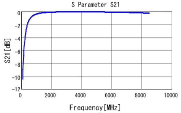
GRM0335C1H5R0BA01 S21 DCOV, 25degC
