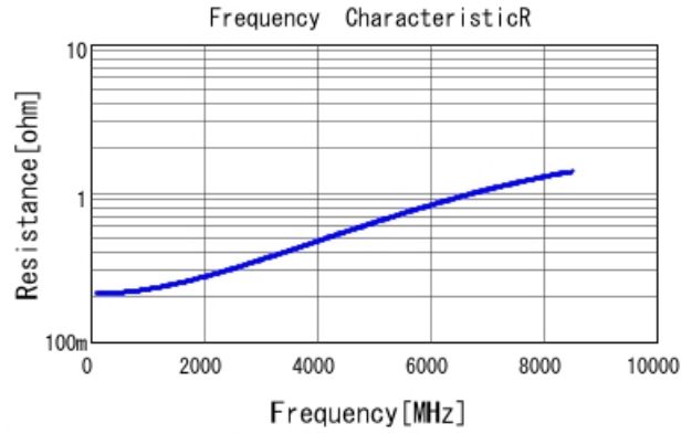
GRM0335C1H5R0BA01 R DCOV, 25degC
