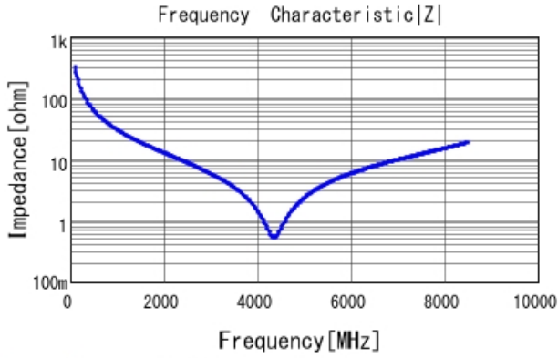
GRM0335C1H5R0BA01 |Z| DCOV, 25degC
