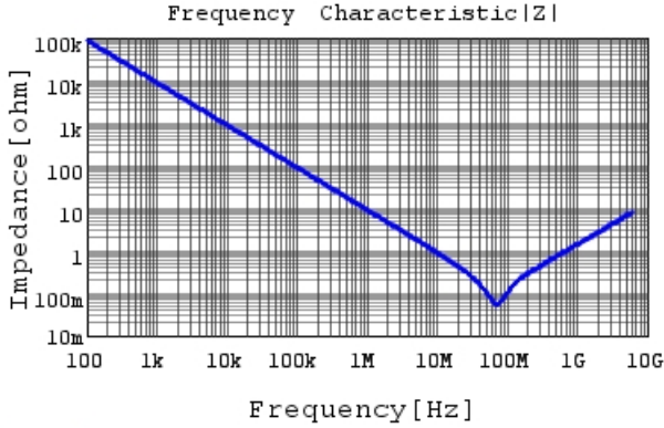
GRM033R61A183KE84 |Z| DCOV, 25degC
