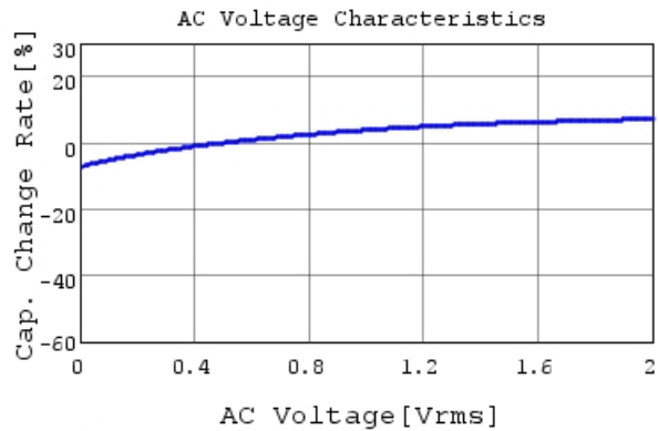
GRM033R61A183KE84 C-AC Voltage capchange, Dc
