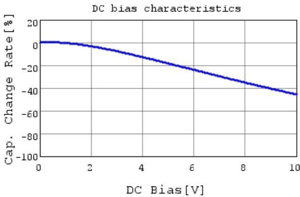
GRM033R61A183KE84 C-DC bias capchange, 25.0c
