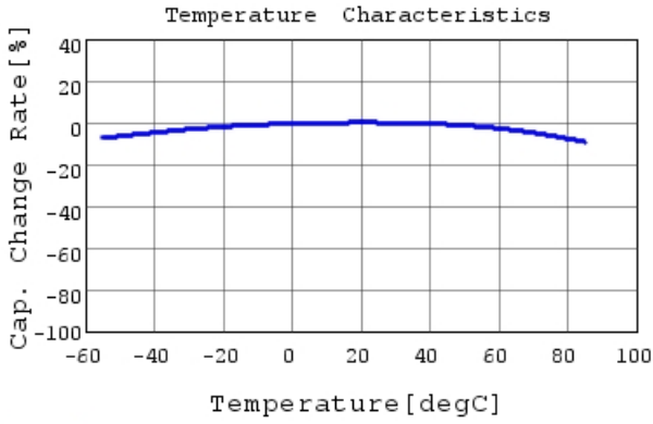
GRM033R61A183KE84 C-Temp. capchange, DC0.0V,
