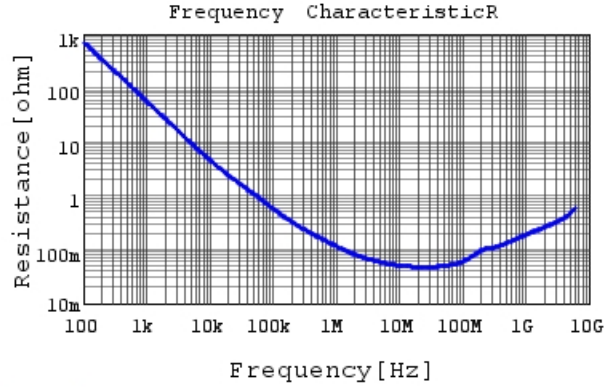
GRM033R61A183KE84 R DCOV, 25degC
