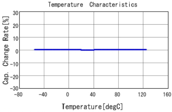
■ GCM1555C1H100JA16 C-Temp. capchange, DCOV, AC1Vrms
