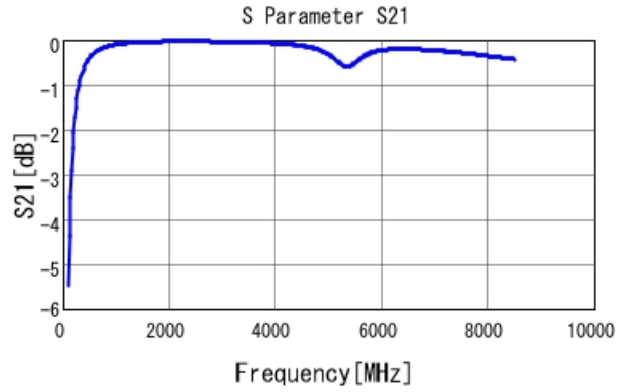
■ GCM1555C1H100JA16 S21 DCOV, 25degC
