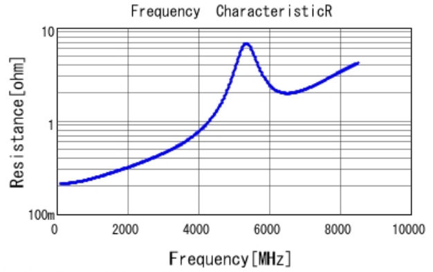
GCM1555C1H100JA16 R DC0V, 25degC
