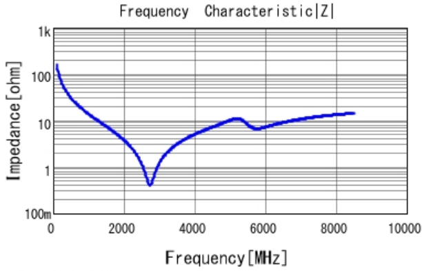
GCM1555C1H100JA16 |Z| DC0V, 25degC
