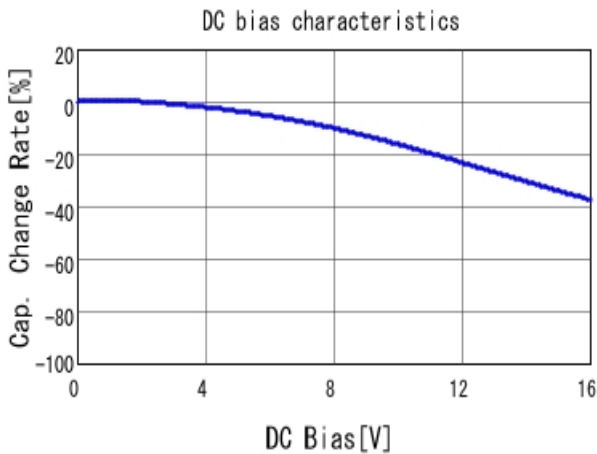
■ GRM31MR11C225KA35 C-DC bias capchange, 20.0degC, AC1.
