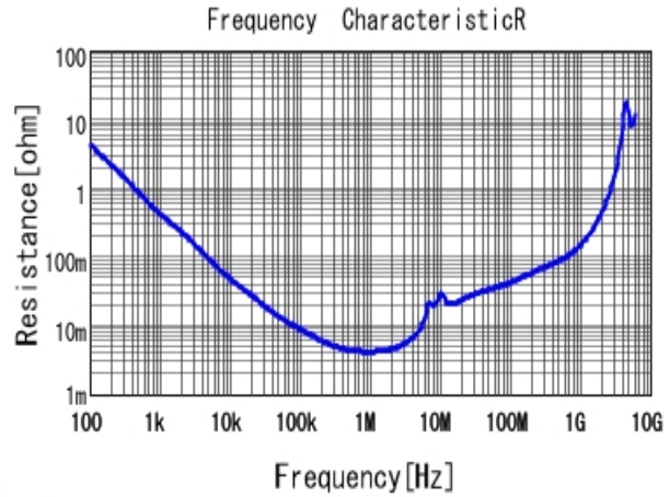
■ GRM31MR11C225KA35 R DCOV, 20degC
