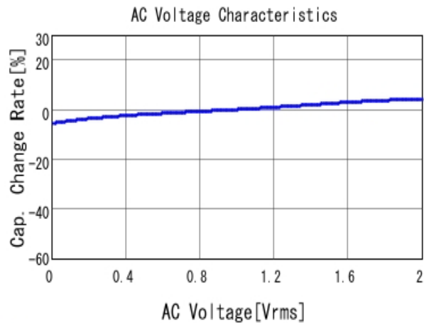
■ GRM31MR11C225KA35 C-AC Voltage capchange, DCOV, 20.0d
