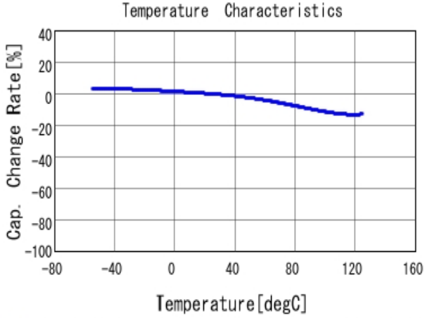
■ GRM31MR11C225KA35 C-Temp. capchange, DC0.0V, AC1.0V r m
