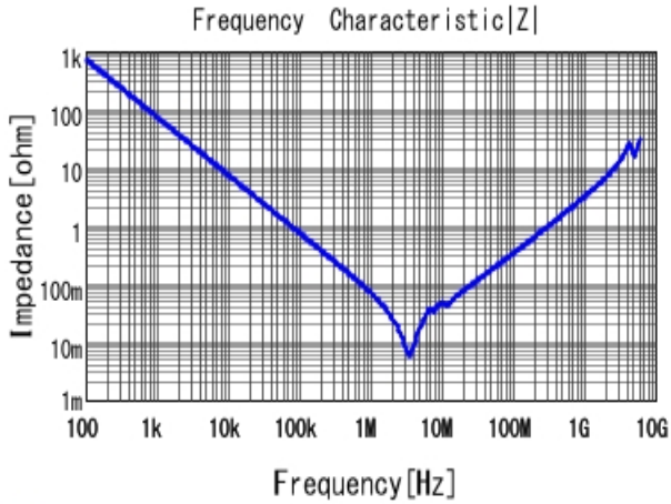
■ GRM31MR11C225KA35 |Z| DCOV, 20degC
