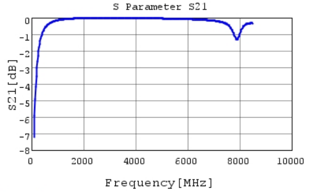
GCQ1555C1H7R7WB01 S21 DCOV, 25degC
