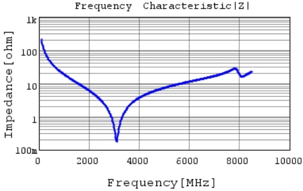
GCQ1555C1H7R7WB01 |Z| DC0V, 25degC
