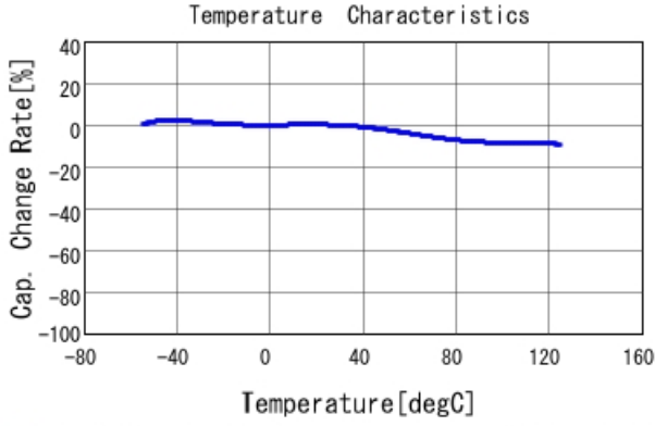
■ GCD188R72A332KA01 C-Temp. capchange, DCO. 0V, AC1. 0V rm
