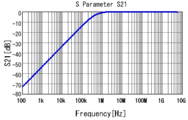
■ GCD188R72A332KA01 S21 DCOV, 25degC
