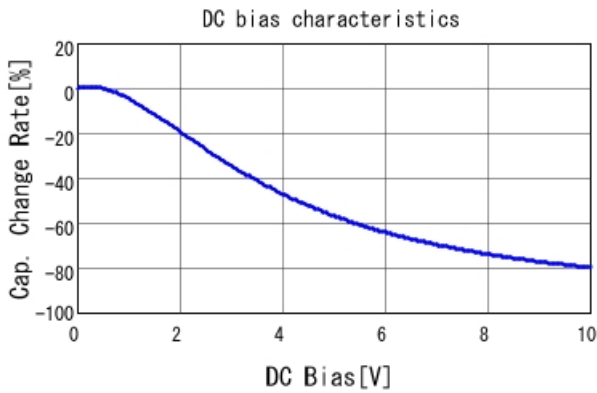
GRM319R61A226ME15 C-DC bias capchange, 25.0degC, A
