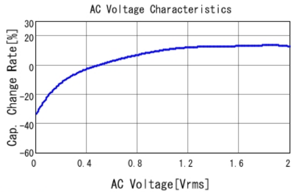
GRM319R61A226ME15 C-AC Voltage capchange, DCOV, 25
