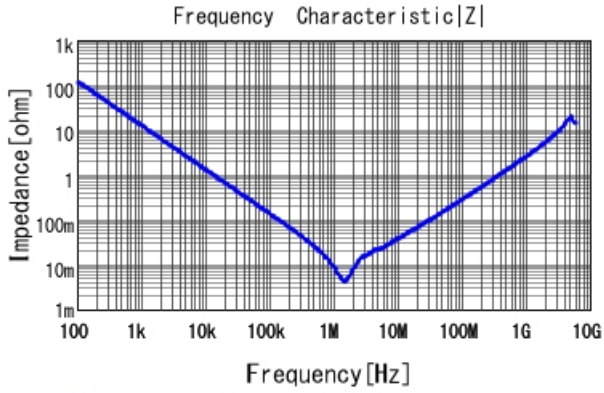
GRM319R61A226ME15 |Z| DCOV, 25degC
