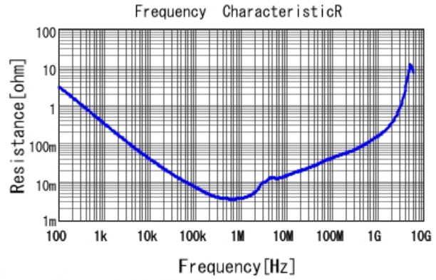
GRM319R61A226ME15 R DCOV, 25degC
