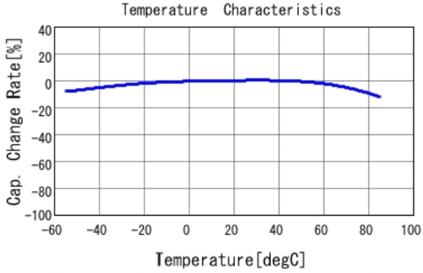
GRM319R61A226ME15 C-Temp. capchange, DC0.0V, ACO.5
