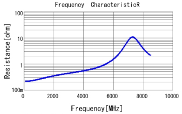
GRM1555C1H5R8BA01 R DCOV, 25degC
