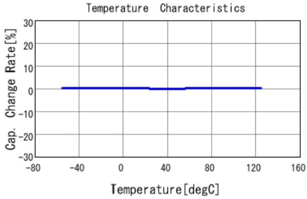
GRM1555C1H5R8BA01 C-Temp. capchange, DC0V, AC1Vrms
