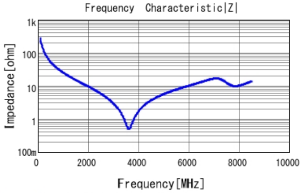
GRM1555C1H5R8BA01 |Z| DCOV, 25degC
