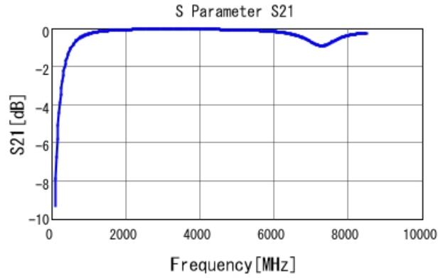
GRM1555C1H5R8BA01 S21 DC0V, 25degC
