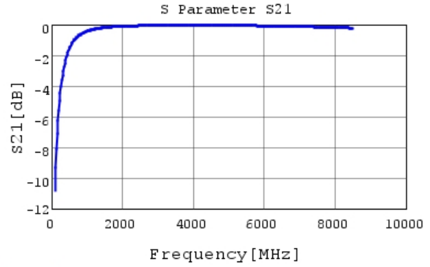
GRM0335C2A4R8CA01 S21 DCOV, 25degC
