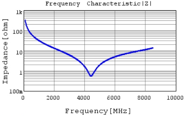
GRM0335C2A4R8CA01 |Z| DCOV, 25degC
