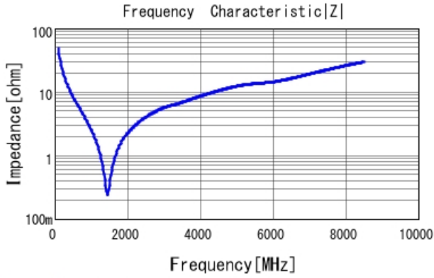
GRM1555C1E330JA01 |Z| DCOV, 25degC
