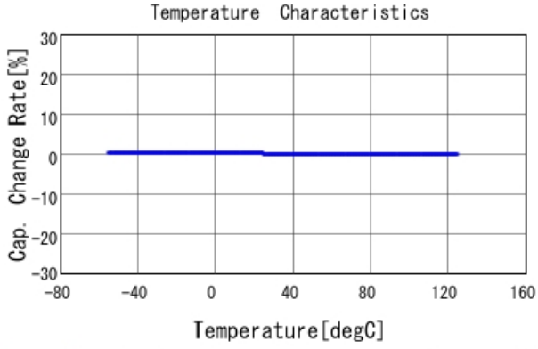
GRM1555C1E330JA01 C-Temp. capchange, DCOV, AC1Vrms
