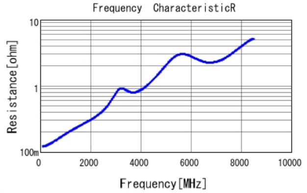
GRM1555C1E330JA01 R DCOV, 25degC
