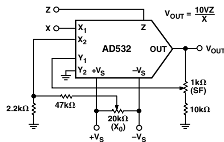
Figure 13. Divider Connection
