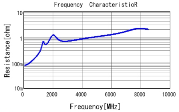
■ GRT1555C1H181JA02 R DC0V, 25degC
