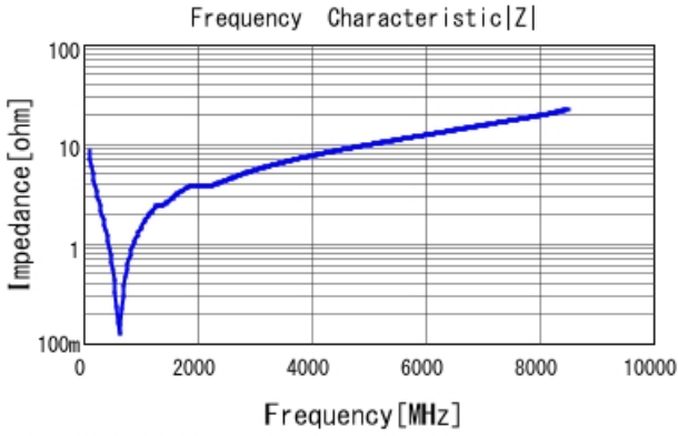
■ GRT1555C1H181JA02 |Z| DC0V, 25degC
