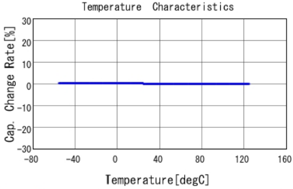
GRM2165C2A181JA01 C-Temp. capchange, DCOV, AC1Vrms
