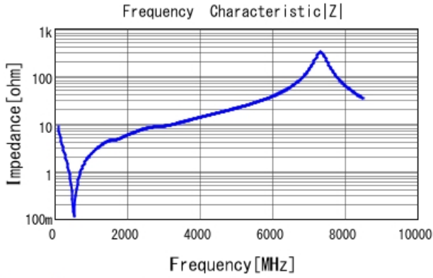
GRM2165C2A181JA01 |Z| DCOV, 25degC
