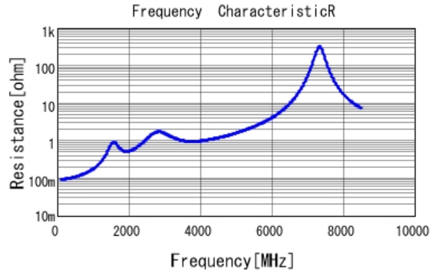
GRM2165C2A181JA01 R DCOV, 25degC
