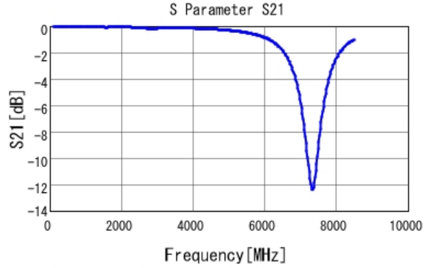
GRM2165C2A181JA01 S21 DCOV, 25degC
