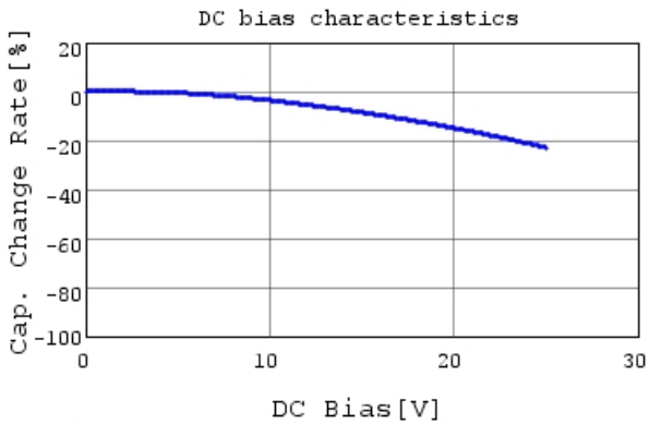
GRM033R61E151KA01 C-DC bias capchange, 25.0c
