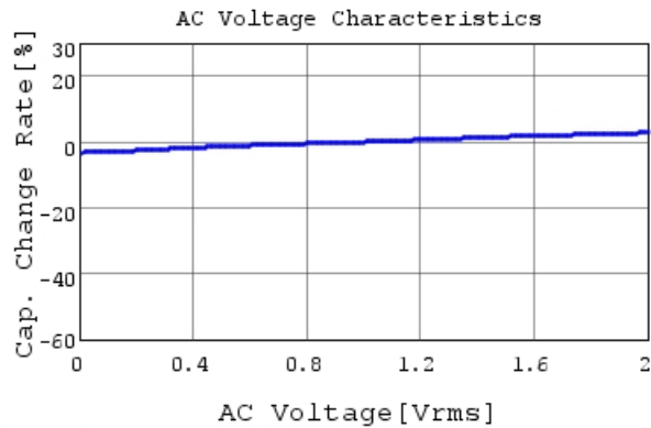
GRM033R61E151KA01 C-AC Voltage capchange, Dc
