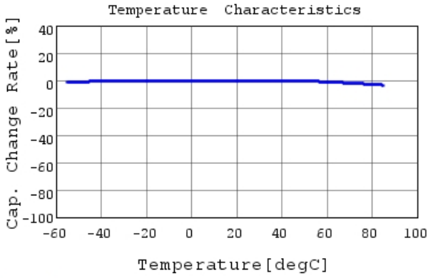
GRM033R61E151KA01 C-Temp. capchange, DC0.0V,
