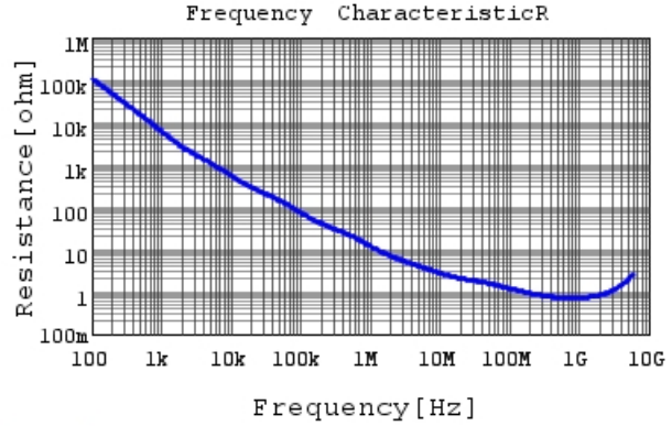
GRM033R61E151KA01 R DCOV, 25degC
