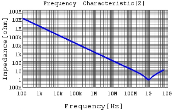
GRM033R61E151KA01 |Z| DCOV, 25degC
