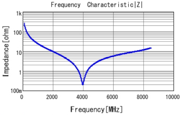
GJM0335C1E6R2CB01 |Z| DCOV, 25degC
