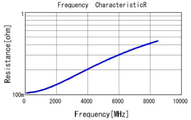
GJM0335C1E6R2CB01 R DCOV, 25degC
