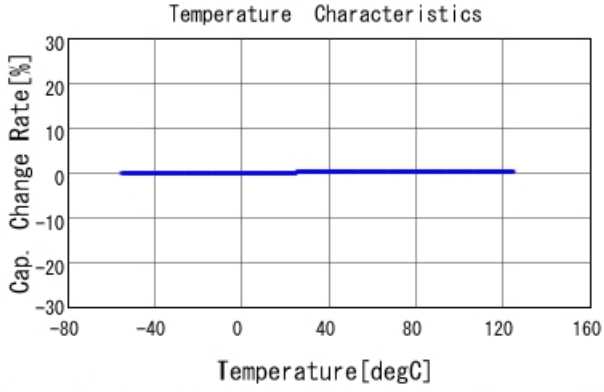
GJM0335C1E6R2CB01 C-Temp. capchange, DC0V, AC1Vrms
