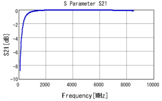
GJM0335C1E6R2CB01 S21 DC0V, 25degC
