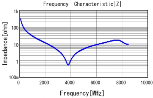
GRM1555C1H5R1WA01 |Z| DCOV, 25degC
