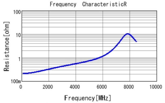
GRM1555C1H5R1WA01 R DCOV, 25degC
