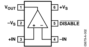
Figure 2. SC70-6 (KS)
