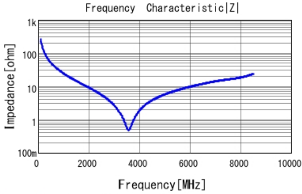
GRM1555C2A6R0DA01 |Z| DCOV, 25degC
