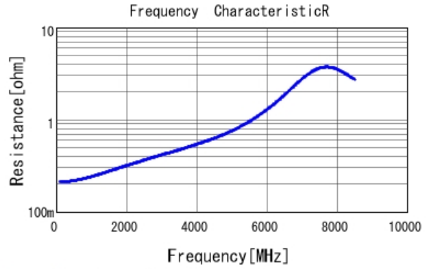
GRM1555C2A6R0DA01 R DCOV, 25degC
