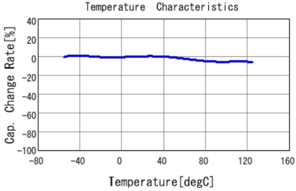
GCJ188R72A102MA01 C-Temp. capchange, DC0.0V, AC1.C
