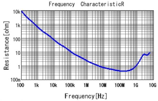
GCJ188R72A102MA01 R DCOV, 25degC
