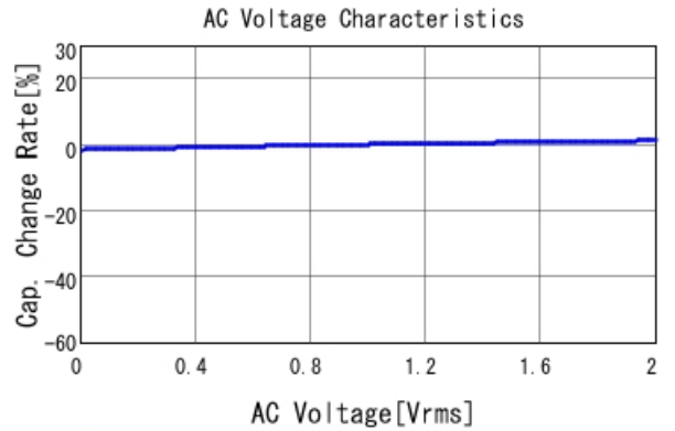
GCJ188R72A102MA01 C-AC Voltage capchange, DCOV, 25
