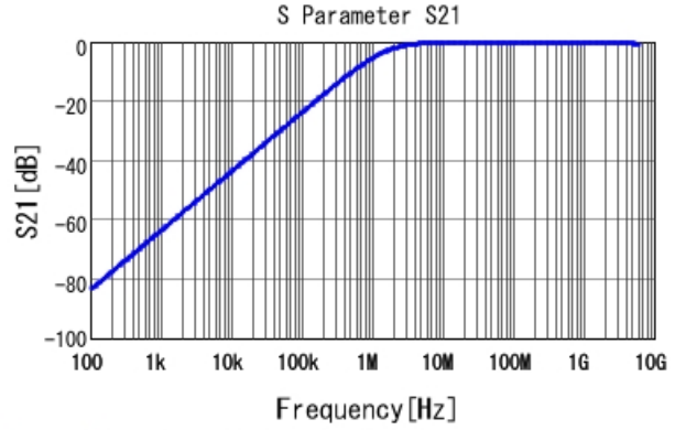
GCJ188R72A102MA01 S21 DC0V, 25degC
