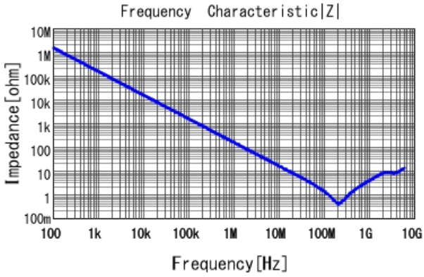
GCJ188R72A102MA01 |Z| DCOV, 25degC
