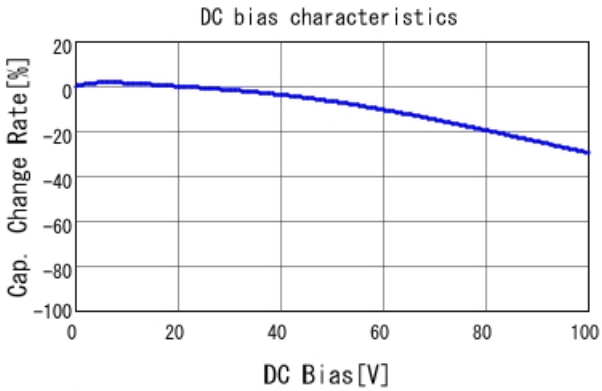
GCJ188R72A102MA01 C-DC bias capchange, 25.0degC, A
