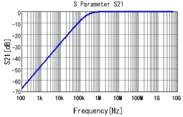
■ GCJ188R71H682KA01 S21 DCOV, 25degC
