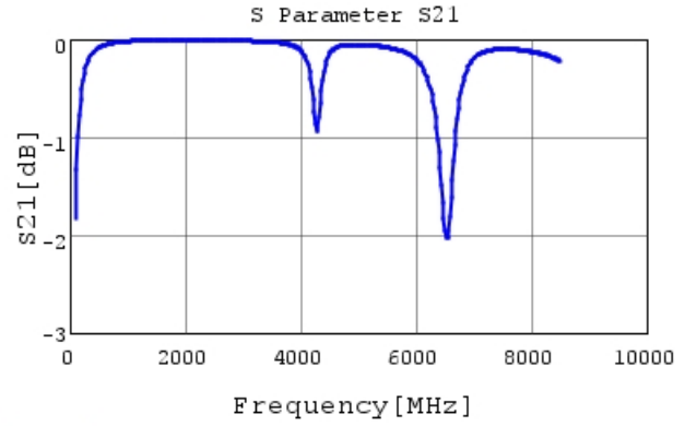
GCQ1555C1H220GB01 S21 DCOV, 25degC
