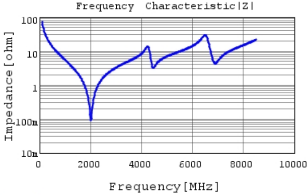
GCQ1555C1H220GB01 |Z| DC0V, 25degC
