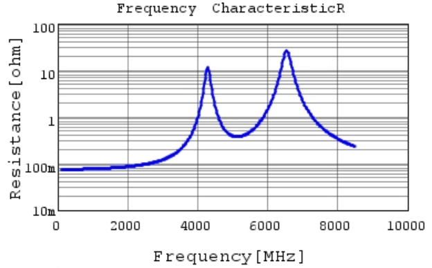
GCQ1555C1H220GB01 R DC0V, 25degC
