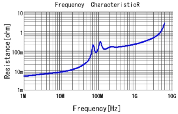
GRM3195C2A303JA01 R DCOV, 25degC
