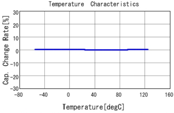
GRM3195C2A303JA01 C-Temp. capchange, DCOV, AC1Vrms
