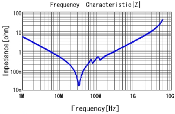
GRM3195C2A303JA01 |Z| DCOV, 25degC
