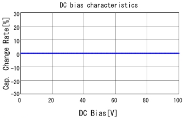
GRM3195C2A303JA01 C-DC bias capchange, 25.0degC, A
