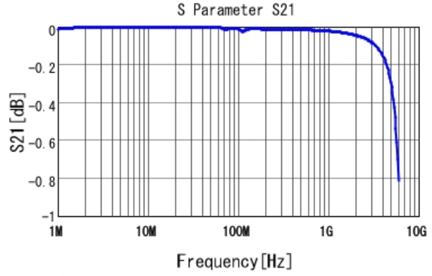
GRM3195C2A303JA01 S21 DCOV, 25degC
