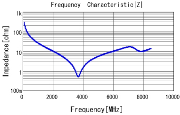
GRM1555C2A5R6WA01 |Z| DCOV, 25degC
