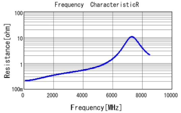
GRM1555C2A5R6WA01 R DCOV, 25degC
