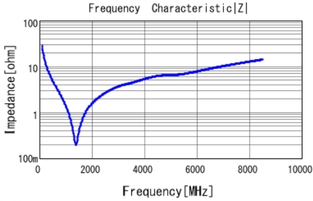
■ GRM0335C2A560JA01 |Z| DCOV, 25degC
