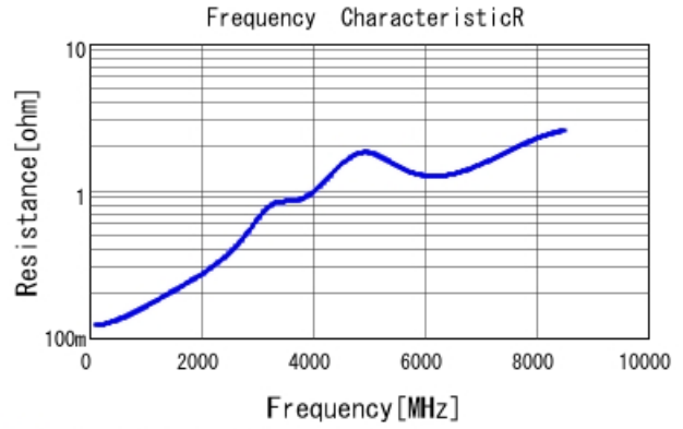
■ GRM0335C2A560JA01 R DCOV, 25degC
