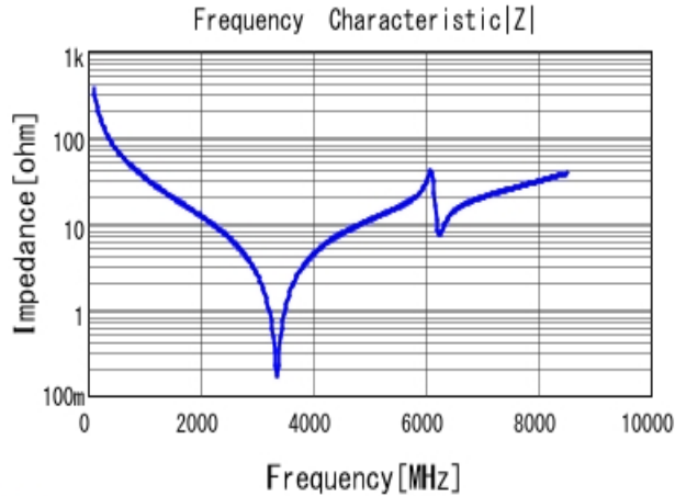
■ GQM1885C2A4R3BB01 |Z| DC0V, 25degC
