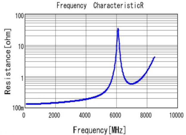
■ GQM1885C2A4R3BB01 R DC0V, 25degC
