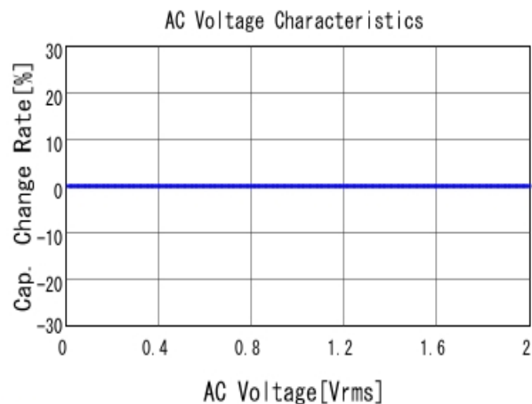
■ GQM1885C2A4R3BB01 C-AC Voltage capchange, DC0V, 25.0d
