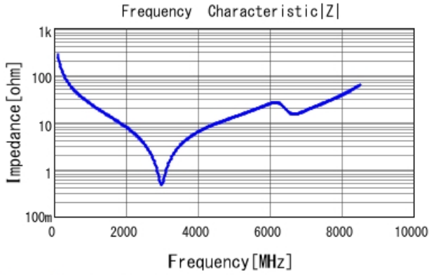
GRM1885C1H5R7DA01 |Z| DCOV, 25degC
