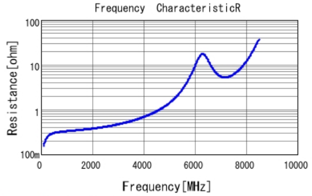
GRM1885C1H5R7DA01 R DCOV, 25degC
