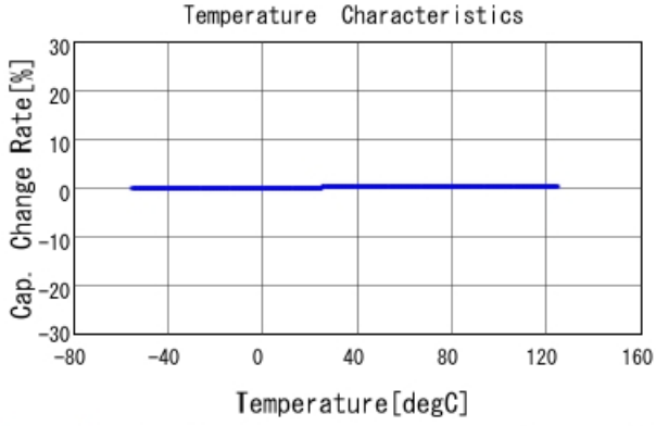
GRM1885C1H5R7DA01 C-Temp. capchange, DCOV, AC1Vrms
