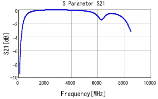
GRM1885C1H5R7DA01 S21 DCOV, 25degC
