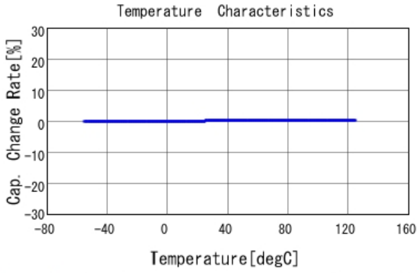
GJM0335C1E5R2BB01 C-Temp. capchange, DC0V, AC1Vrms
