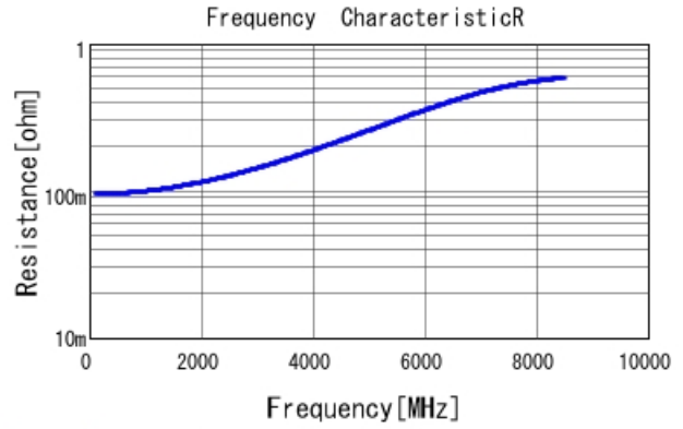
GJM0335C1E5R2BB01 R DC0V, 25degC
