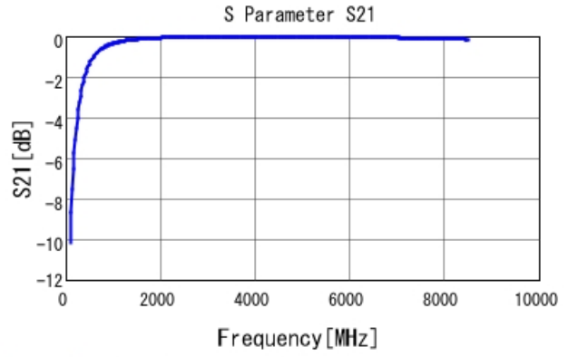
GJM0335C1E5R2BB01 S21 DC0V, 25degC
