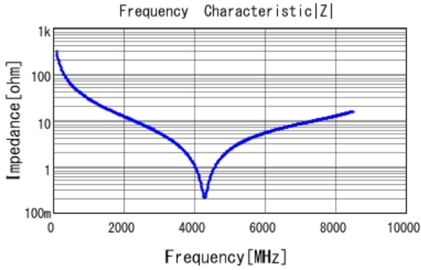
GJM0335C1E5R2BB01 |Z| DC0V, 25degC
