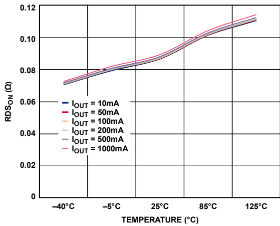
Figure 6. R_{DS(on)} vs. Temperature, LFCSP
