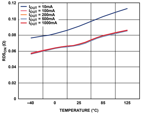
Figure 5. R_{DS(on)} vs. Temperature, WLCSPP
