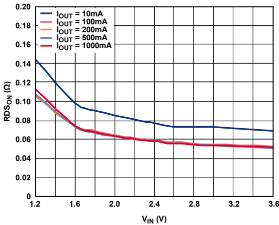
Figure 7. R_{DS(on)} vs. Input Voltage ( V_{IN} ), WLCSPP
