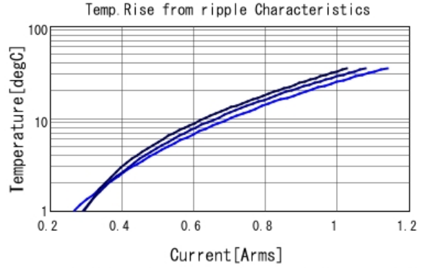
GQM2195G2H3R0BB12 Temp. rise — 1GHz — 2GHz
