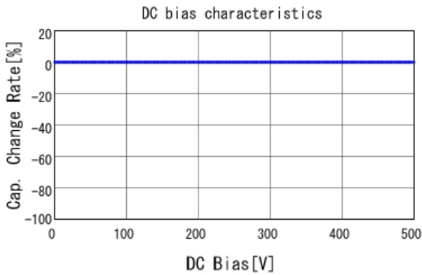
GQM2195G2H3R0BB12 C-DC bias capchange, 25.0degC, A
