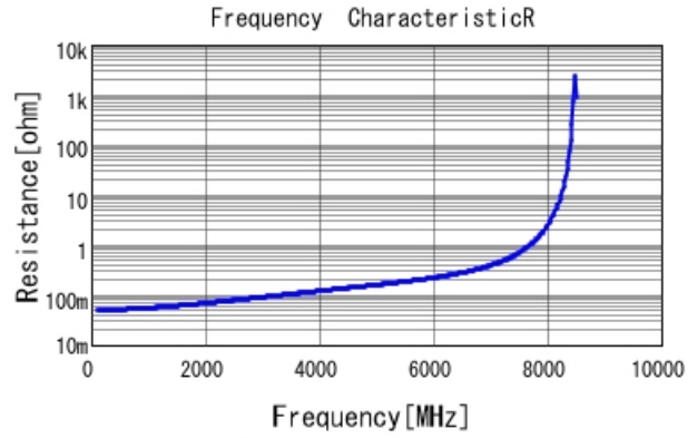
GQM2195G2H3R0BB12 R DCOV, 25degC
