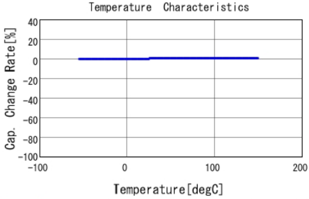
GQM2195G2H3R0BB12 C-Temp. capchange, DCOV, AC1Vrms
