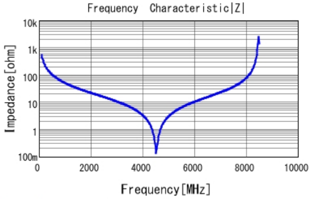
GQM2195G2H3R0BB12 |Z| DCOV, 25degC
