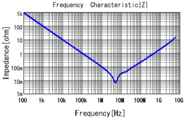
■ GRM188Z71E225KE43 |Z| DCOV, 25degC
