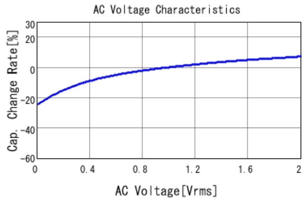
■ GRM188Z71E225KE43 C-AC Voltage capchange, DCOV, 25.0d
