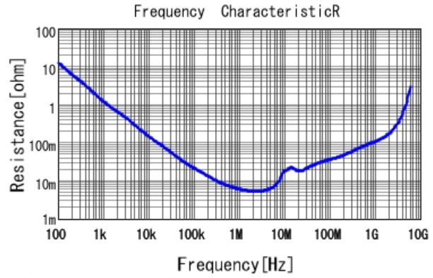
■ GRM188Z71E225KE43 R DCOV, 25degC
