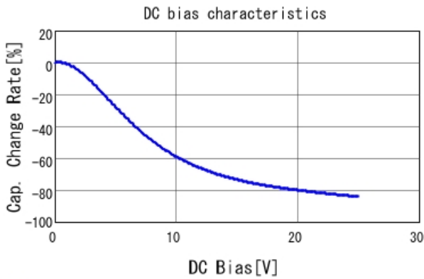
■ GRM188Z71E225KE43 C-DC bias capchange, 25.0degC, AC1V
