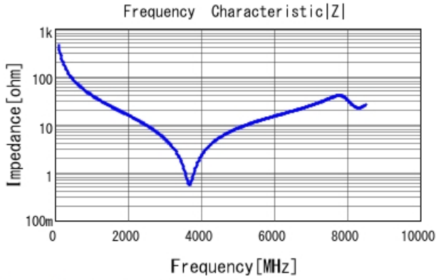
GRM1885C1H3R6BA01 |Z| DCOV, 25degC
