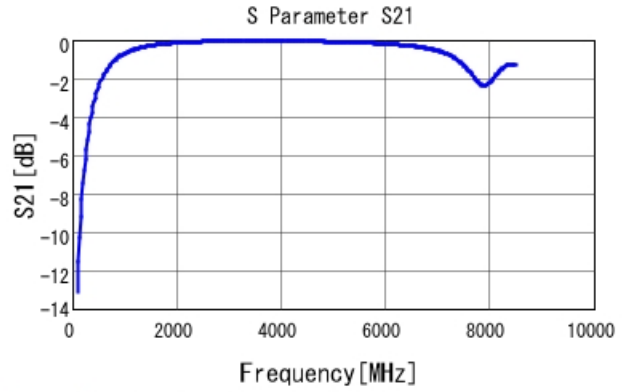
GRM1885C1H3R6BA01 S21 DCOV, 25degC
