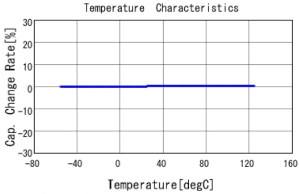
GRM1885C1H3R6BA01 C-Temp. capchange, DCOV, AC1Vrms
