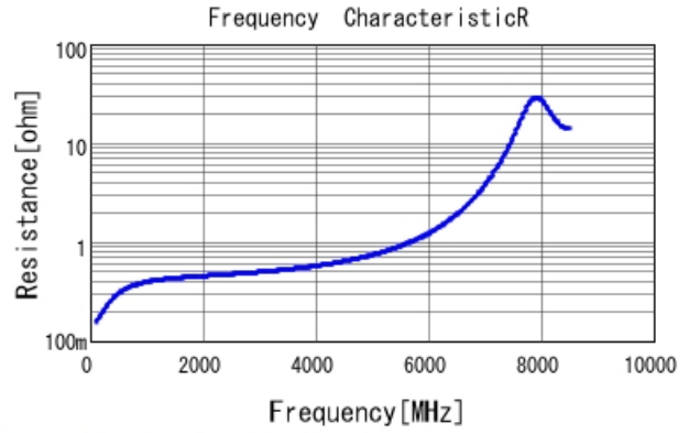
GRM1885C1H3R6BA01 R DCOV, 25degC
