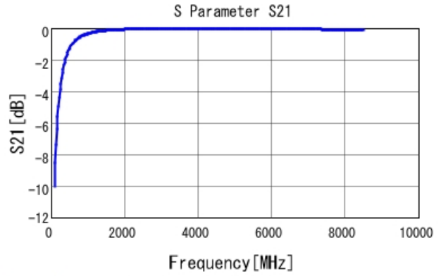
GJM0335C1E5R3WB01 S21 DC0V, 25degC
