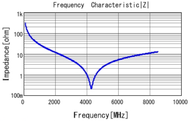
GJM0335C1E5R3WB01 |Z| DCOV, 25degC
