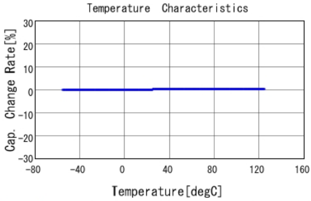
GJM0335C1E5R3WB01 C-Temp. capchange, DC0V, AC1Vrms
