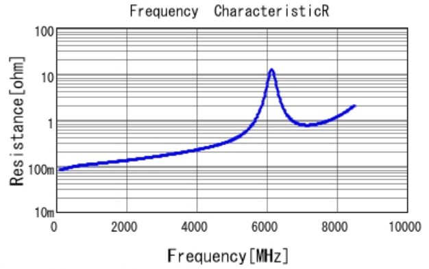
GJM1555C1H130GB01 R DCOV, 25degC
