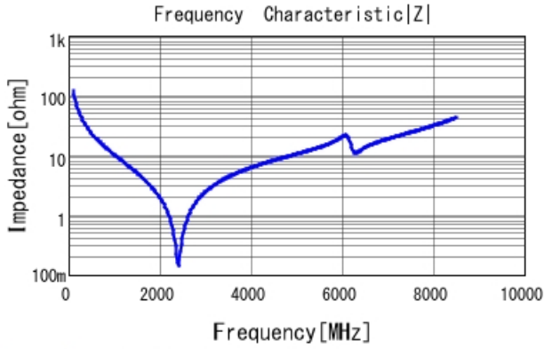
GJM1555C1H130GB01 |Z| DCOV, 25degC
