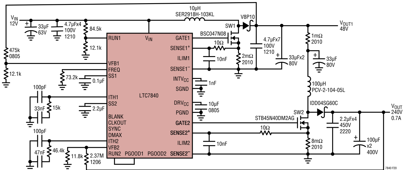
Figure 20. 12V Input, 240V/0.7A Output Two-Stage Boost Converter
