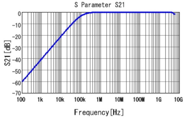
■ GCD188R72A153KA01 S21 DCOV, 25degC
