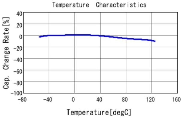
■ GCD188R72A153KA01 C-Temp. capchange, DCO. 0V, AC1. 0Vrm
